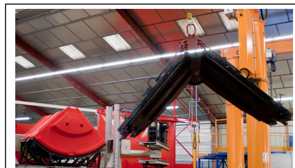
Figure 13: Opened mould
