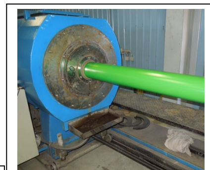
Figure 34: Extrusion process
