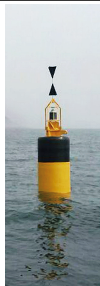
Figure 60: Elastomer buoy with self contained lantern
